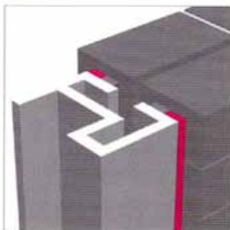
Perimeter Sealing PVC Frames
